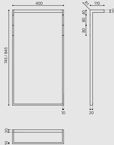
TOWEL RAIL FOR VANITY UNIT WITH ROUND WASHBASIN TOALLERO PARA MUEBLE CON LAVABO REDONDO
